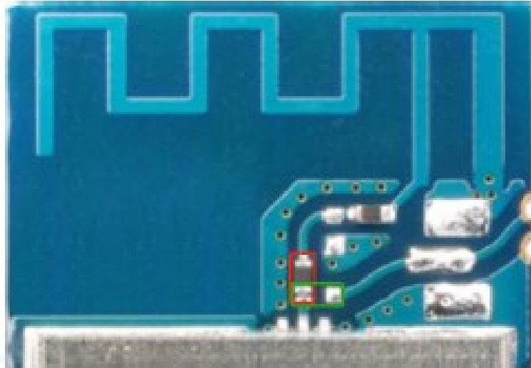
Figure 5. Antenna Output Mode Modification of RF-BM-2652P2(I)
