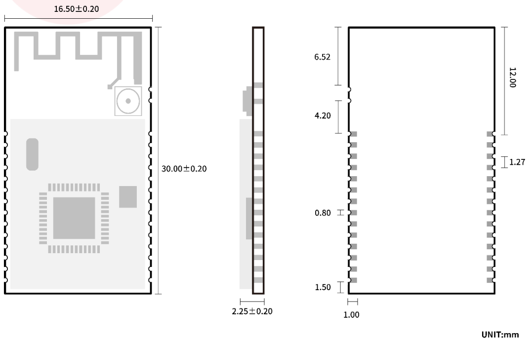
Figure 4. Recommended PCB Footprint of RF-BM-2652P2(I)
