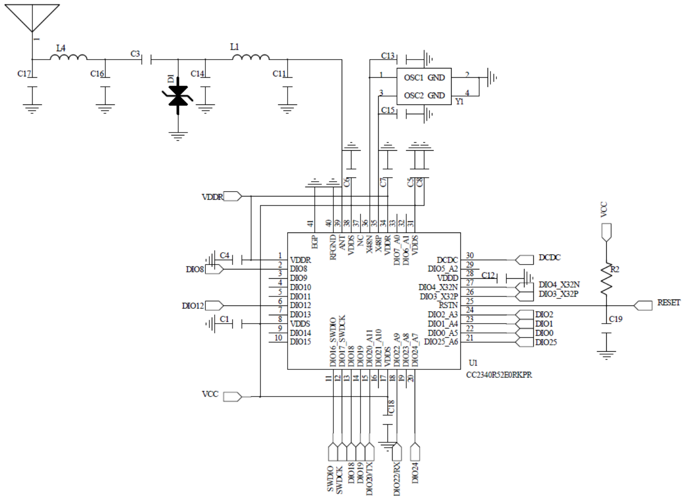
Figure 5. Schematic Diagram of RF-BM-2340T3
